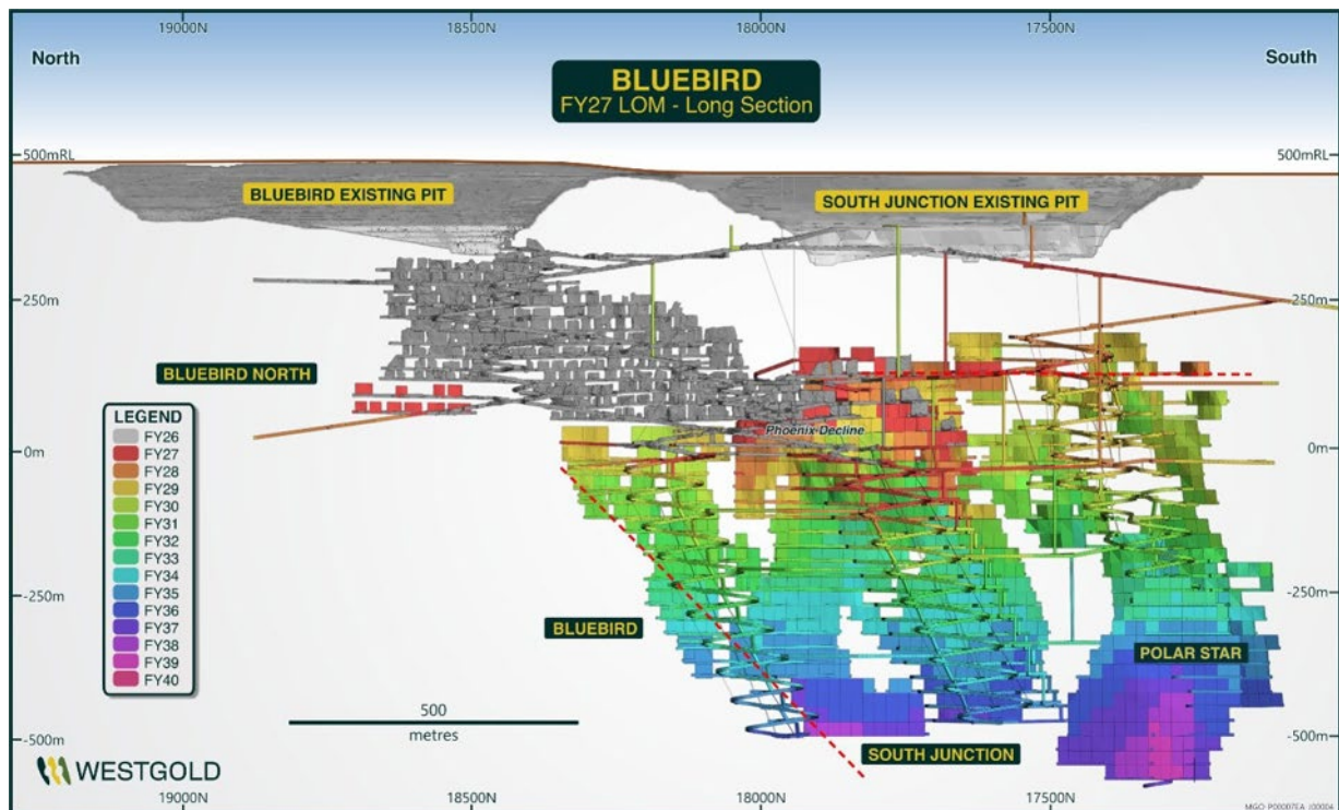
Figure 6: Bluebird-South Junction Long Section
